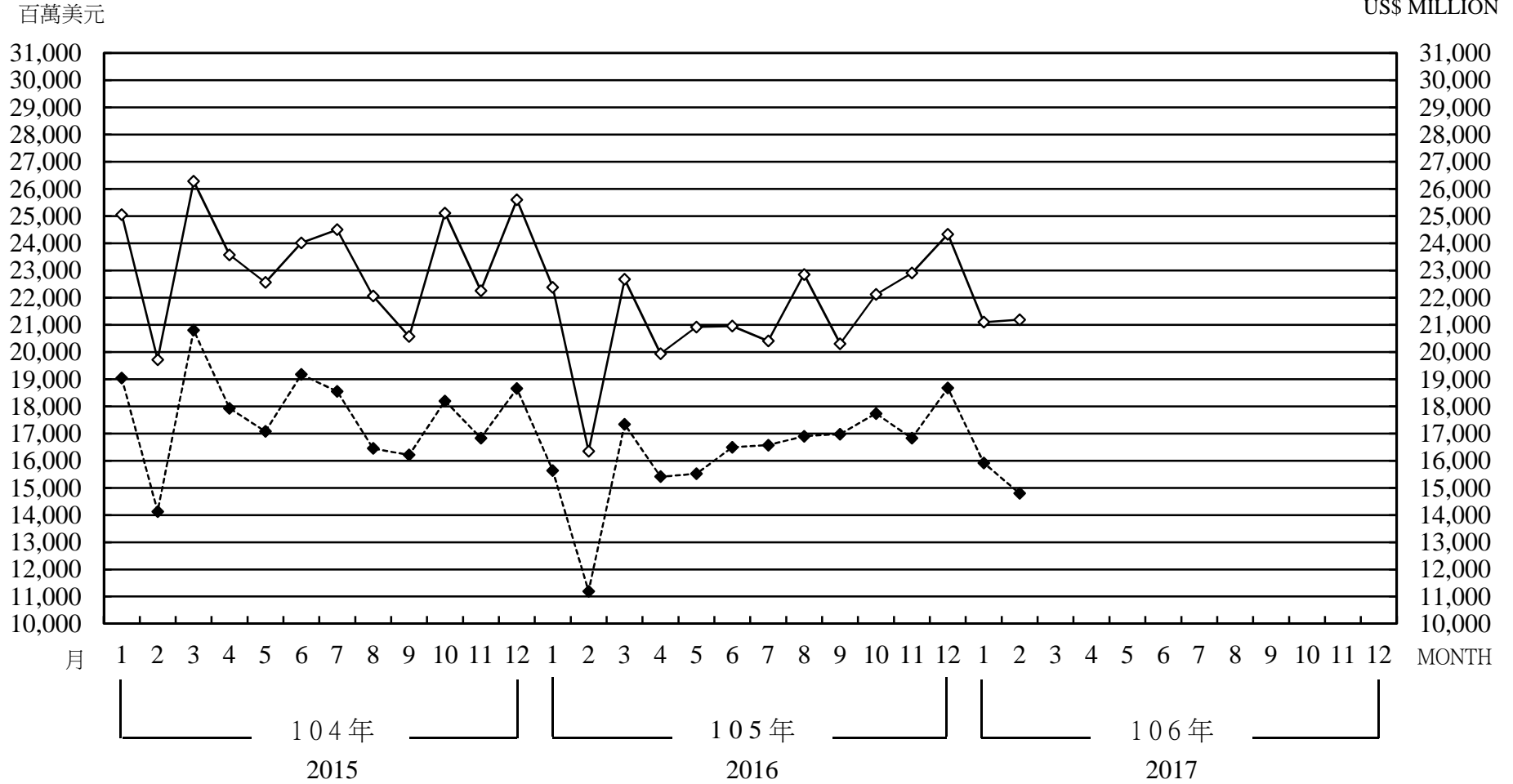
CHART 1 COMPARISON OF FOREIGN EXCHANGE EXPORT PROCEEDS AND IMPORT PAYMENTS (2015-2017)
